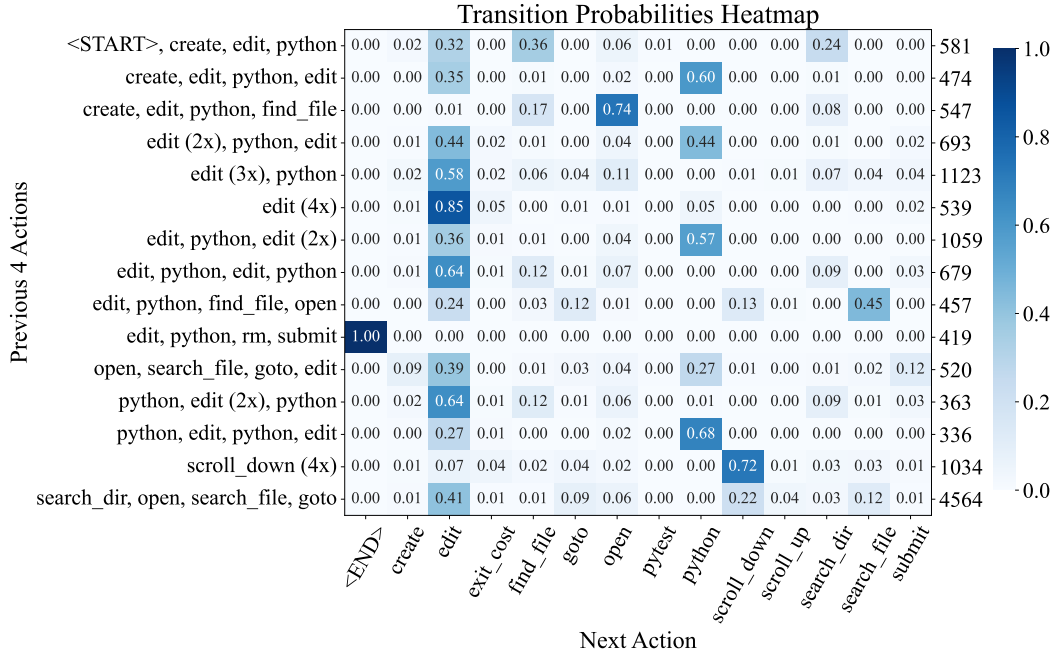
Figure 24: Heatmap displaying the relative frequency of different actions being invoked after the most popular quadruplets of actions in SWE-agent w/ GPT-4 Turbo trajectories across all task instances.
