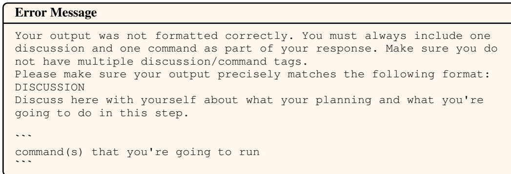
Figure 32: The environment’s error message. This is emitted if a model generation doesn’t conform to the thought-action format suggested.
