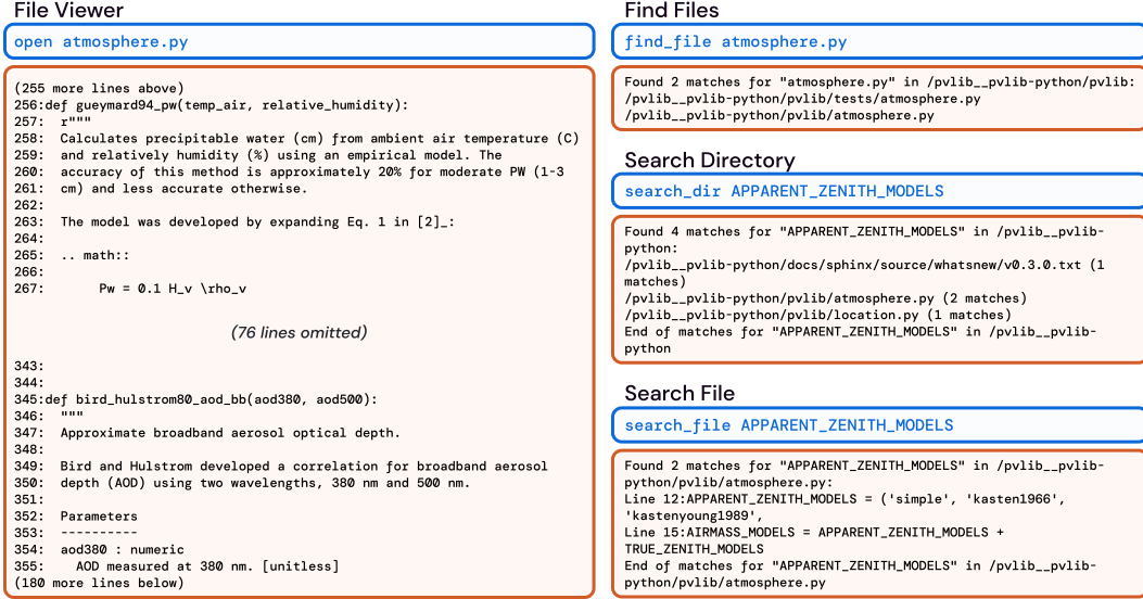
Figure 10: The File Viewer and Search components of the SWE-agent interface. The corresponding commands for each component are shown in blue. These examples are copied from trajectories generated by SWE-agent w/ GPT-4 Turbo on the pvlb__pvlb-python-1603 task instance.
